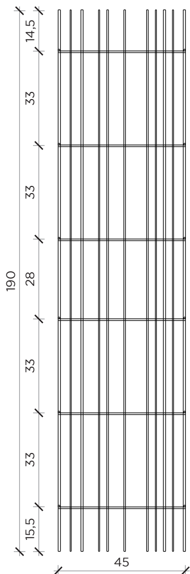
FRONTE | FRONT
