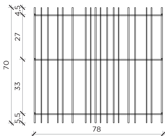
FRONTE | FRONT
