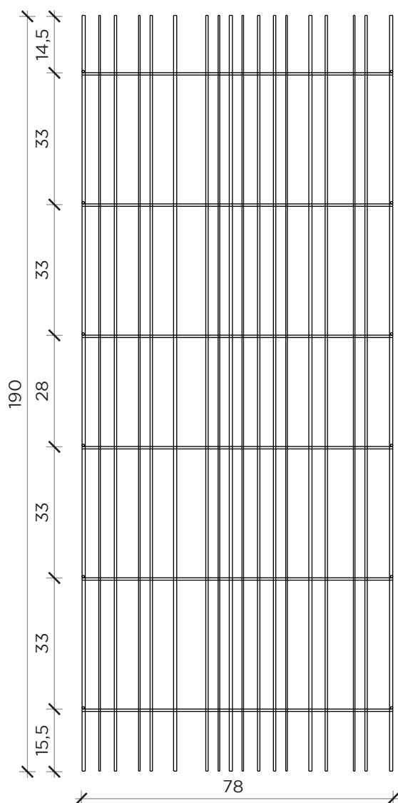
FRONTE | FRONT
