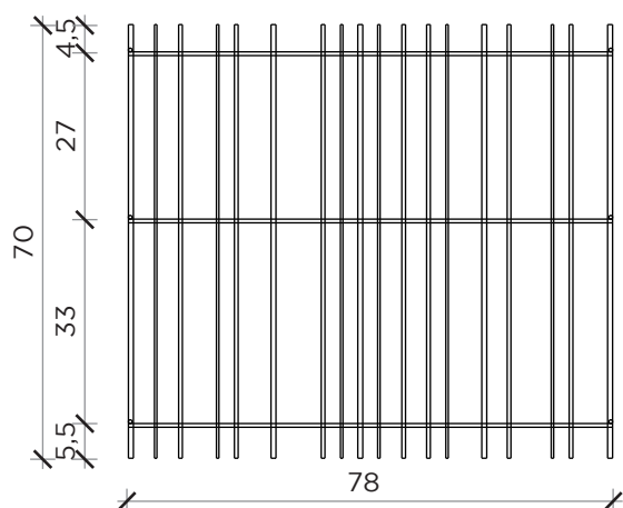
FRONTE | FRONT
