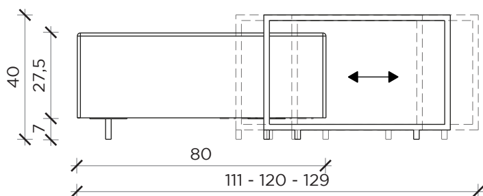
FRONTE | FRONT
