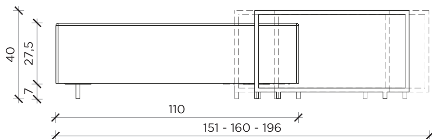
FRONTE | FRONT
